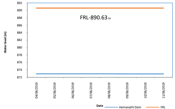
Water Level of Hemavathy Dam Monsoon-2019
