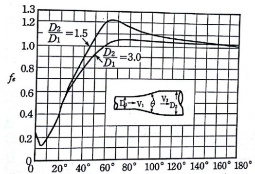
Figure 3.7 Enlargement loss, f_e (Experimental Values by Gibson)
