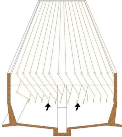
Figure 6.13 Lamella clarifier
