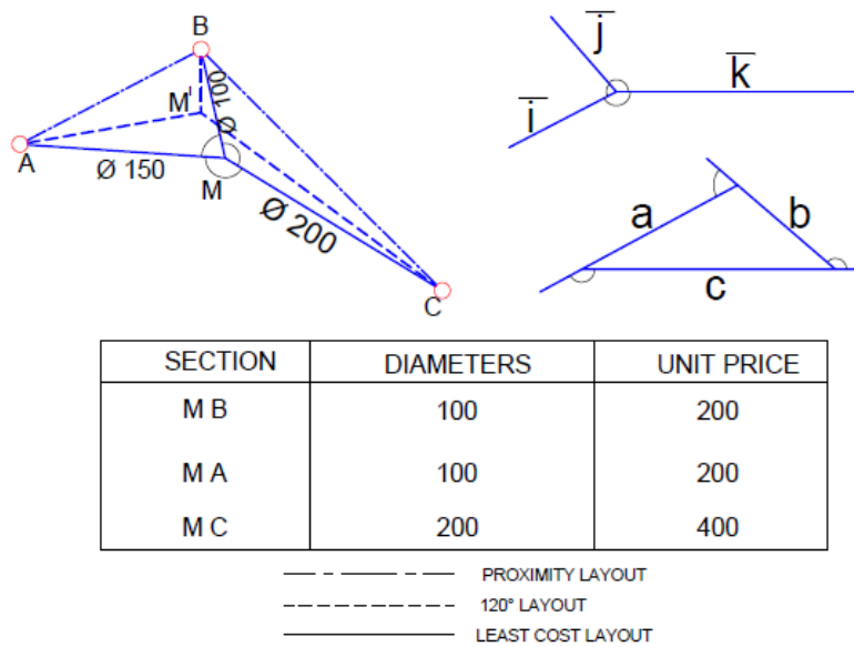
Figure 5.11 Least Count Layout
