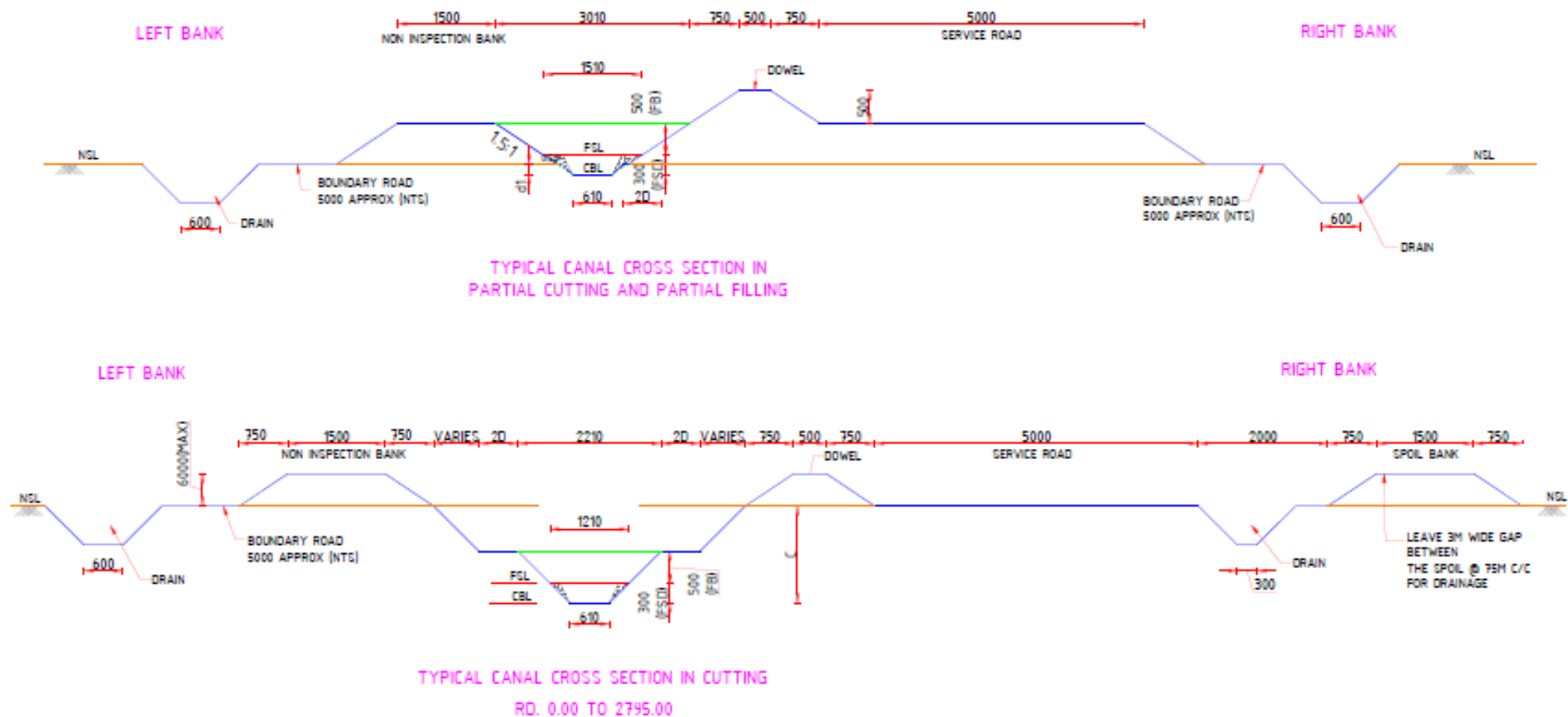
Figure 10.5 Canal Cross-sections
