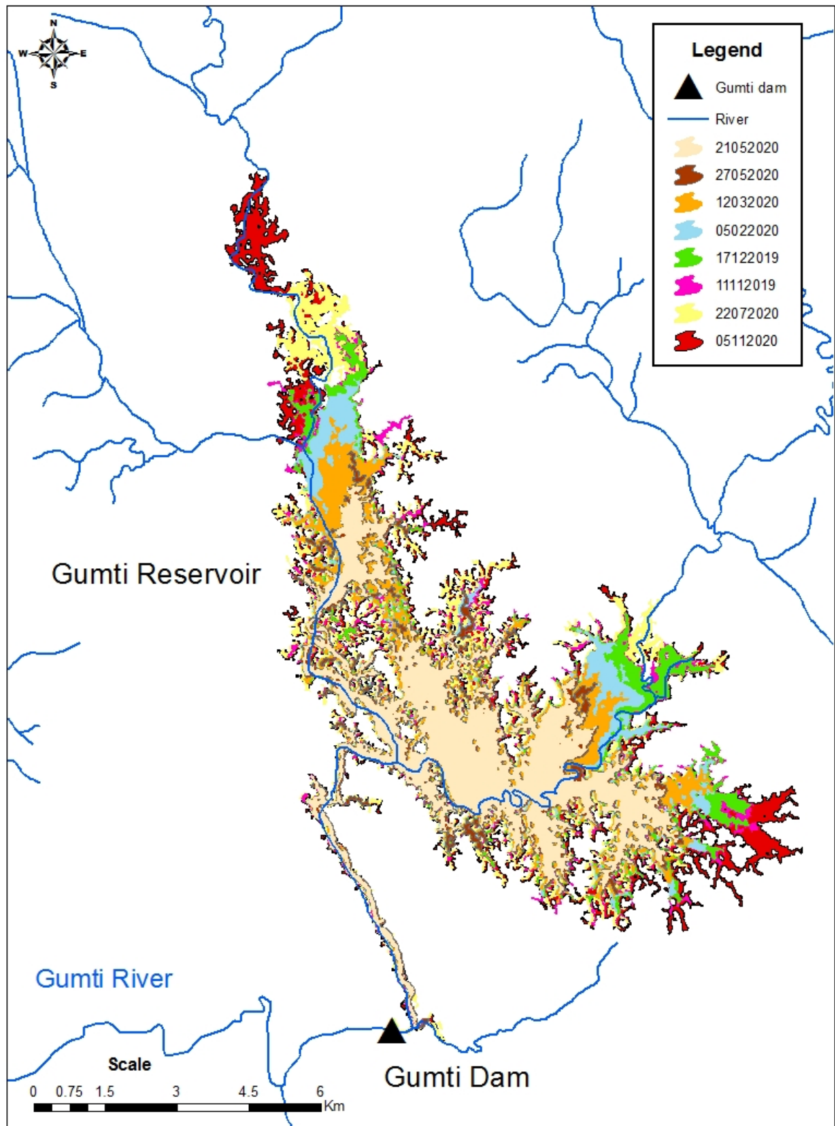
Fig. 7: Water Spread Area of Gumti Reservoir on different dates
