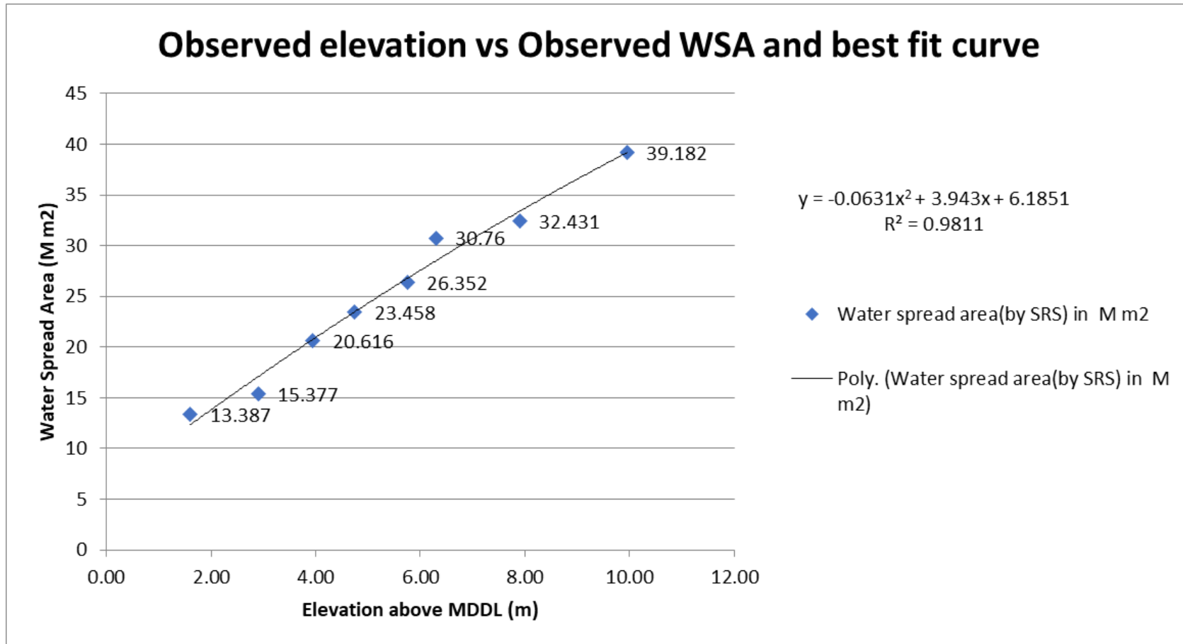
Fig. 8: Observed elevation vs Observed WSA of Gumti Reservoir
