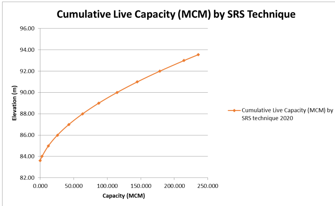
Fig. 9: Modified live capacity - elevation curve (SRS technique)-Gumti reservoir, Tripura
