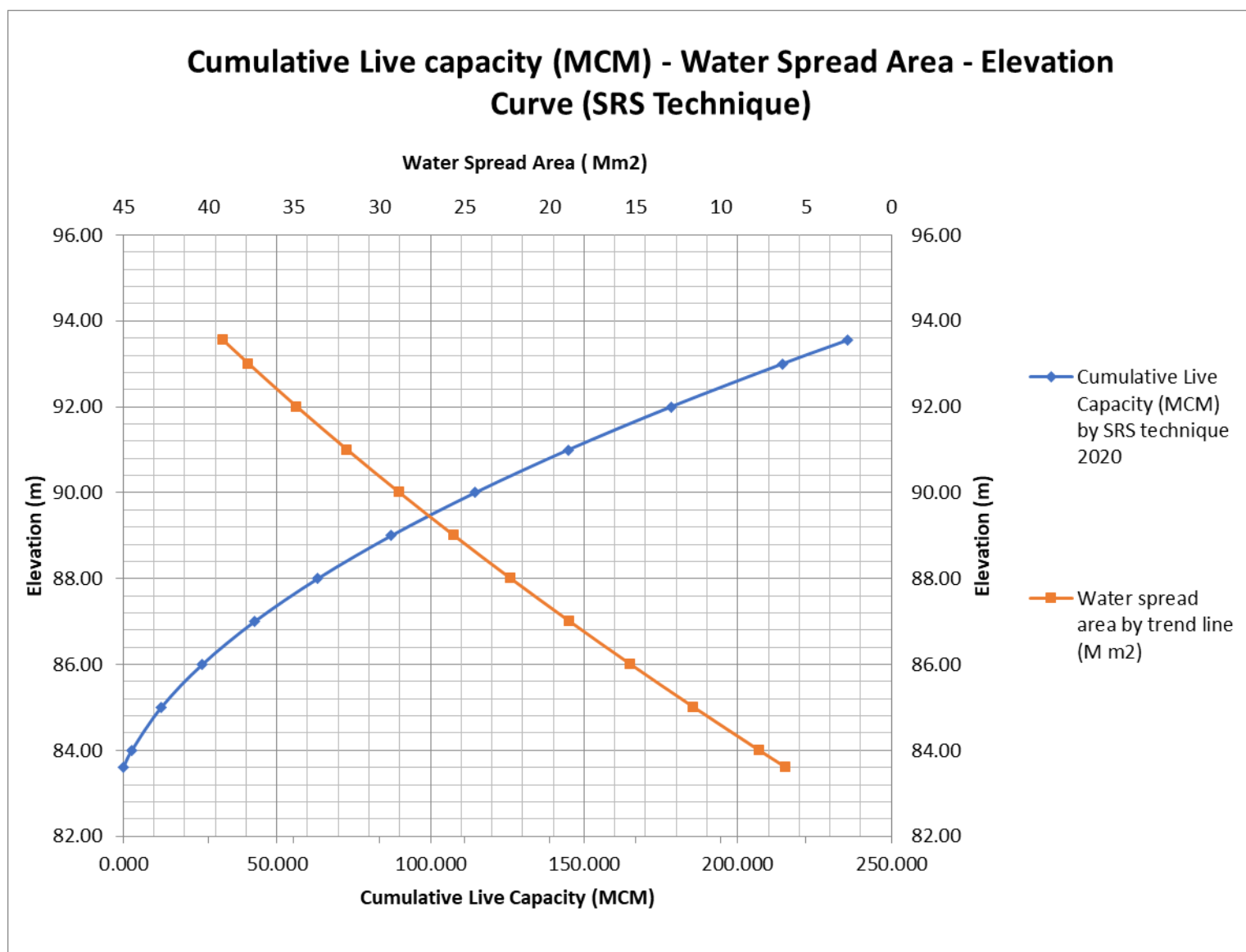
Fig. 10: Elevation – Area- Capacity Curve- Gumti reservoir, Tripura
