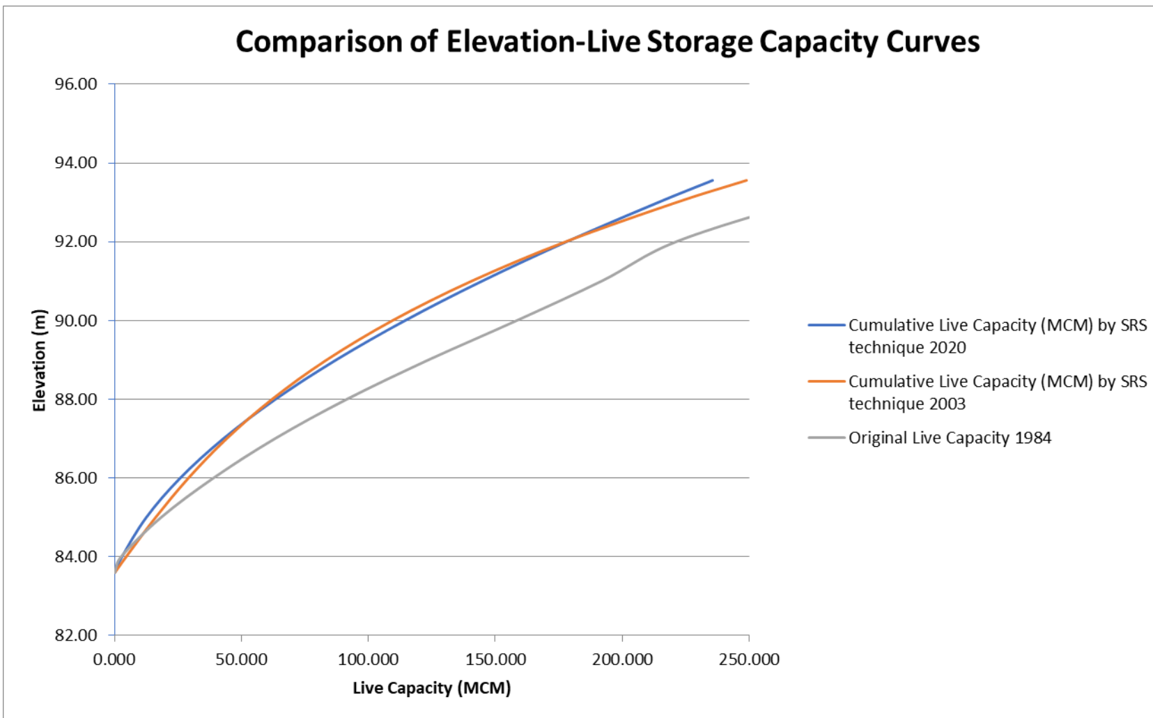
Fig. 11: Comparison of Elevation-Live Storage Capacity Curves (MCM)- Gumti reservoir, Tripura
