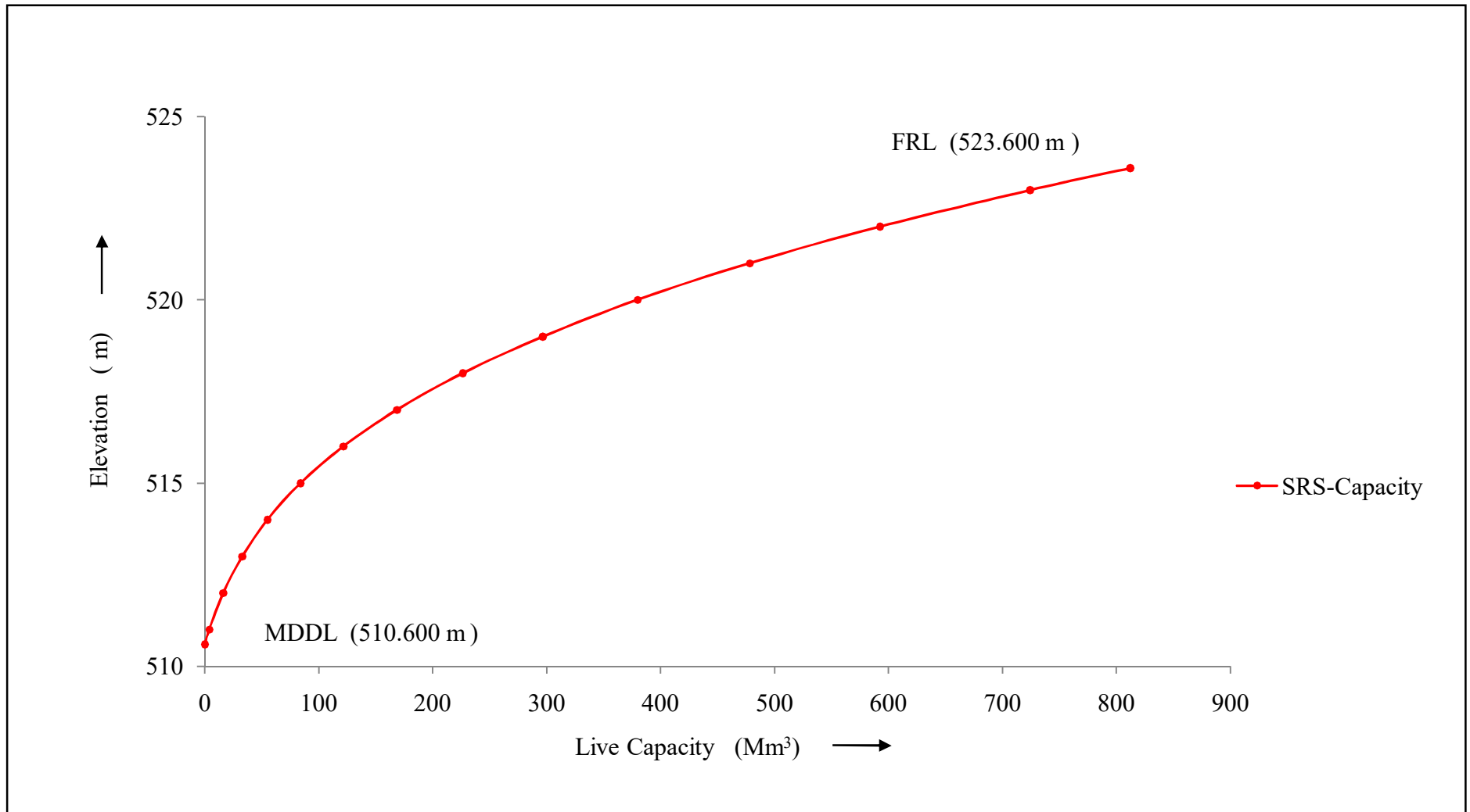
Figure 9 : SRS Elevation-Capacity curve for Singur reservoir, Telangana
