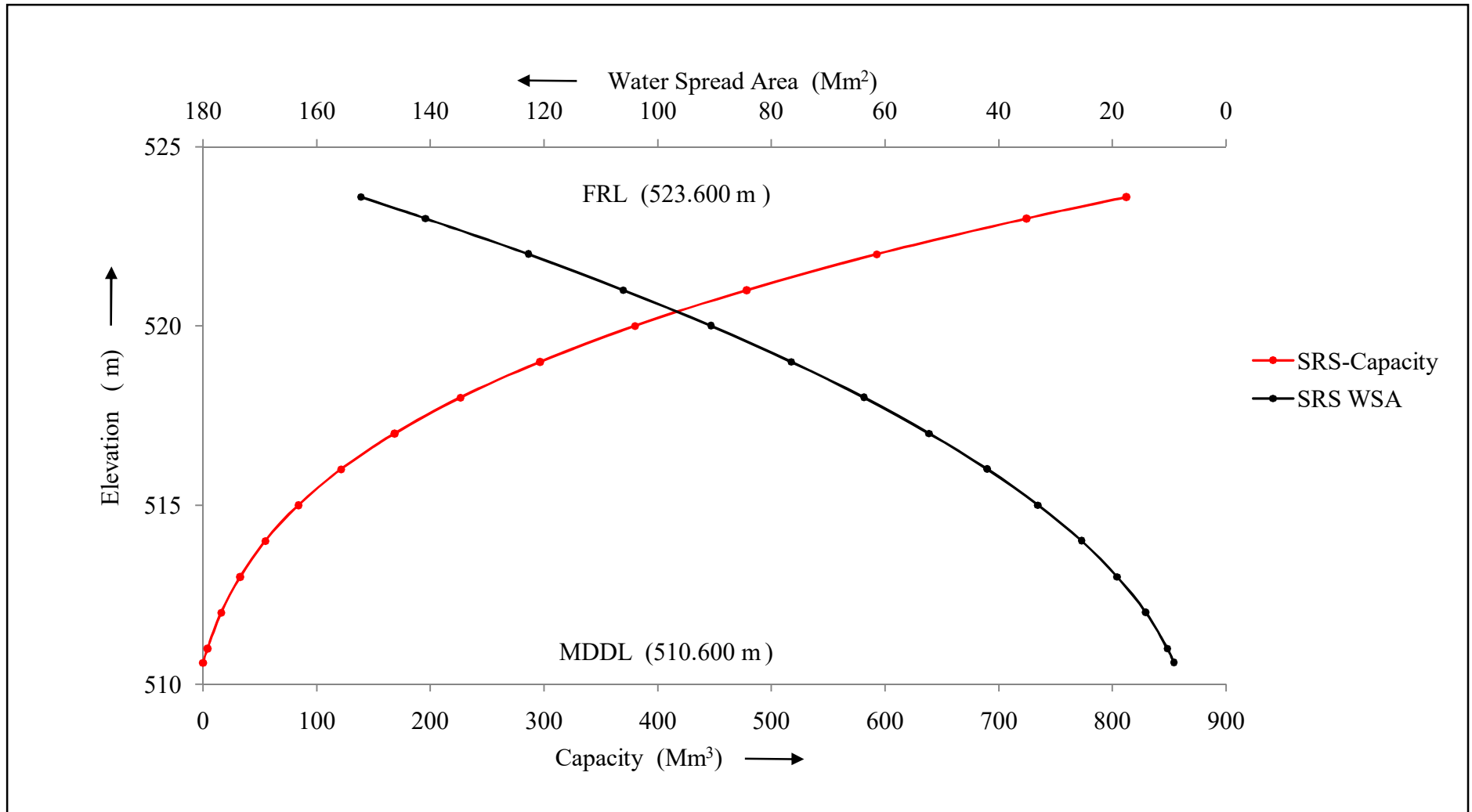
Figure 12 : Modified SRS Elevation-Area-Capacity curve for Singur reservoir, Telangana
