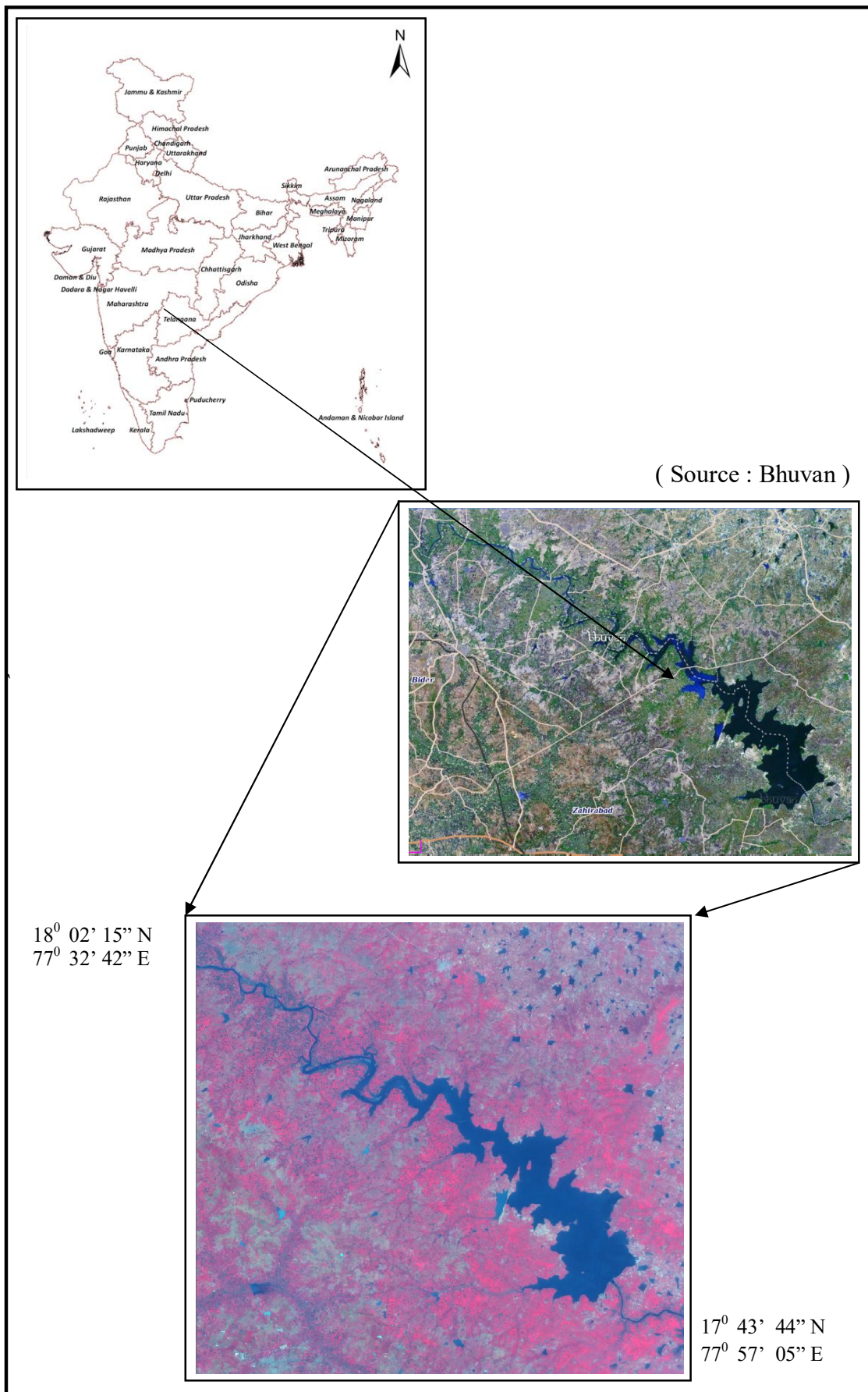
Figure 4 : Index map of Singur reservoir, Telangana
