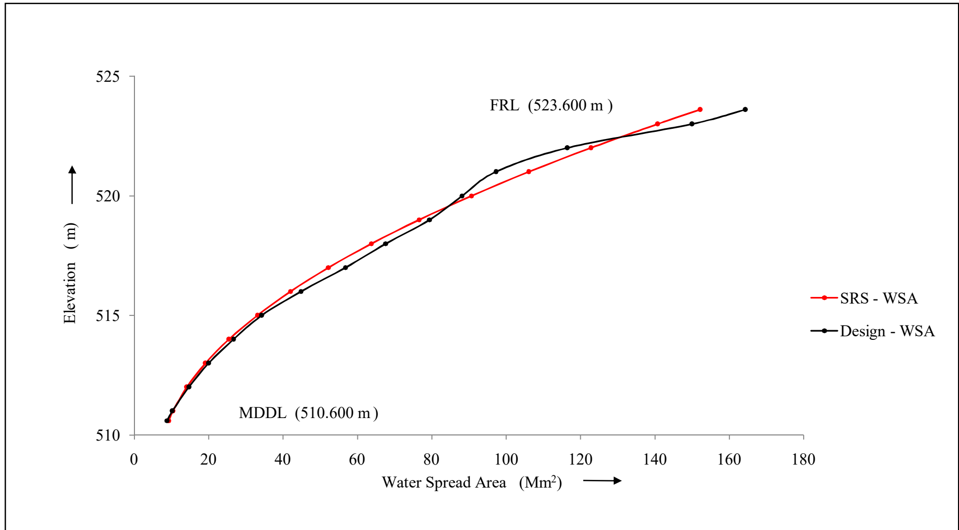
Figure 10 : Elevation-Area curve for different years for Singur reservoir, Telangana
