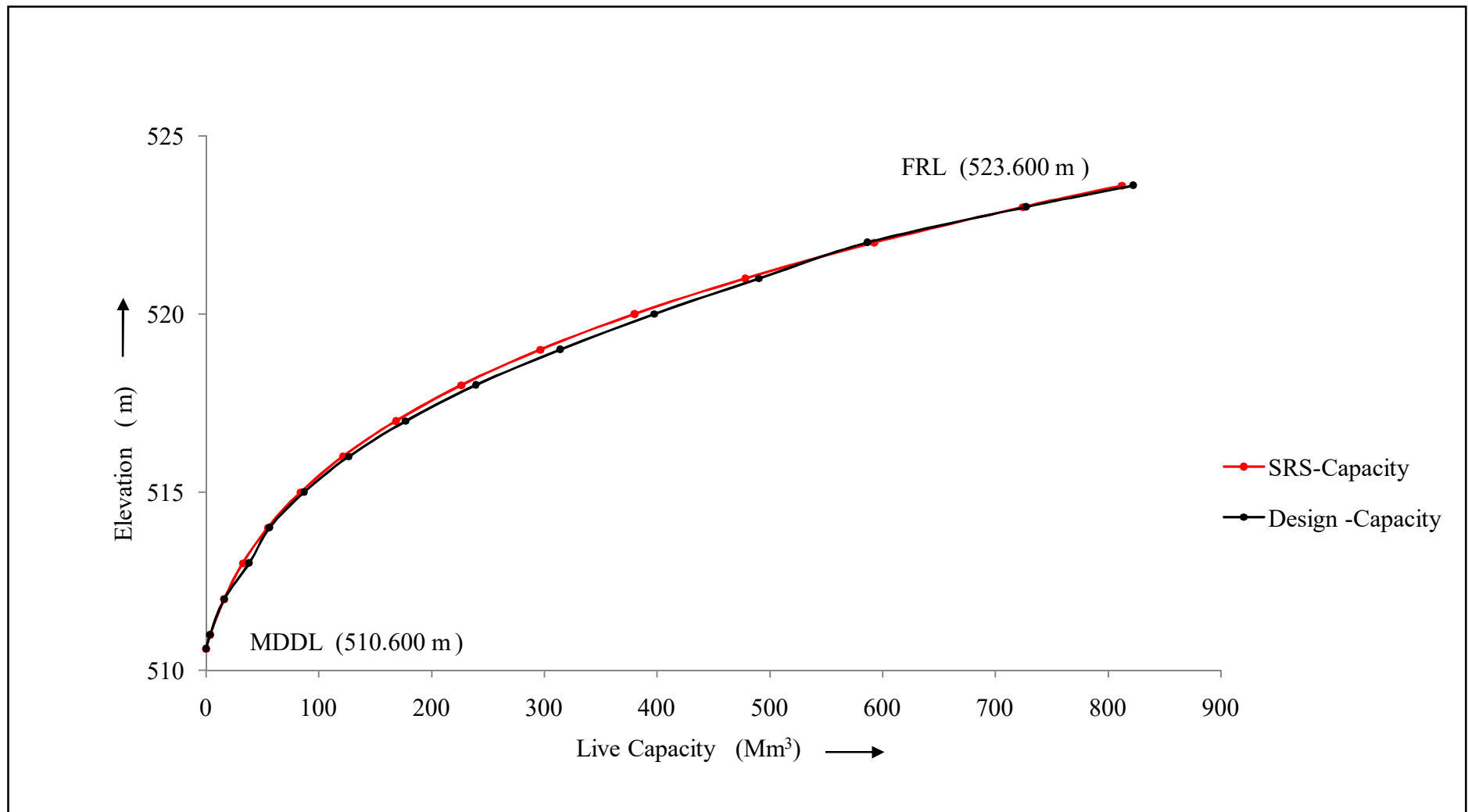
Figure 11 : Elevation-Capacity curve for different years for Singur reservoir, Telangana
