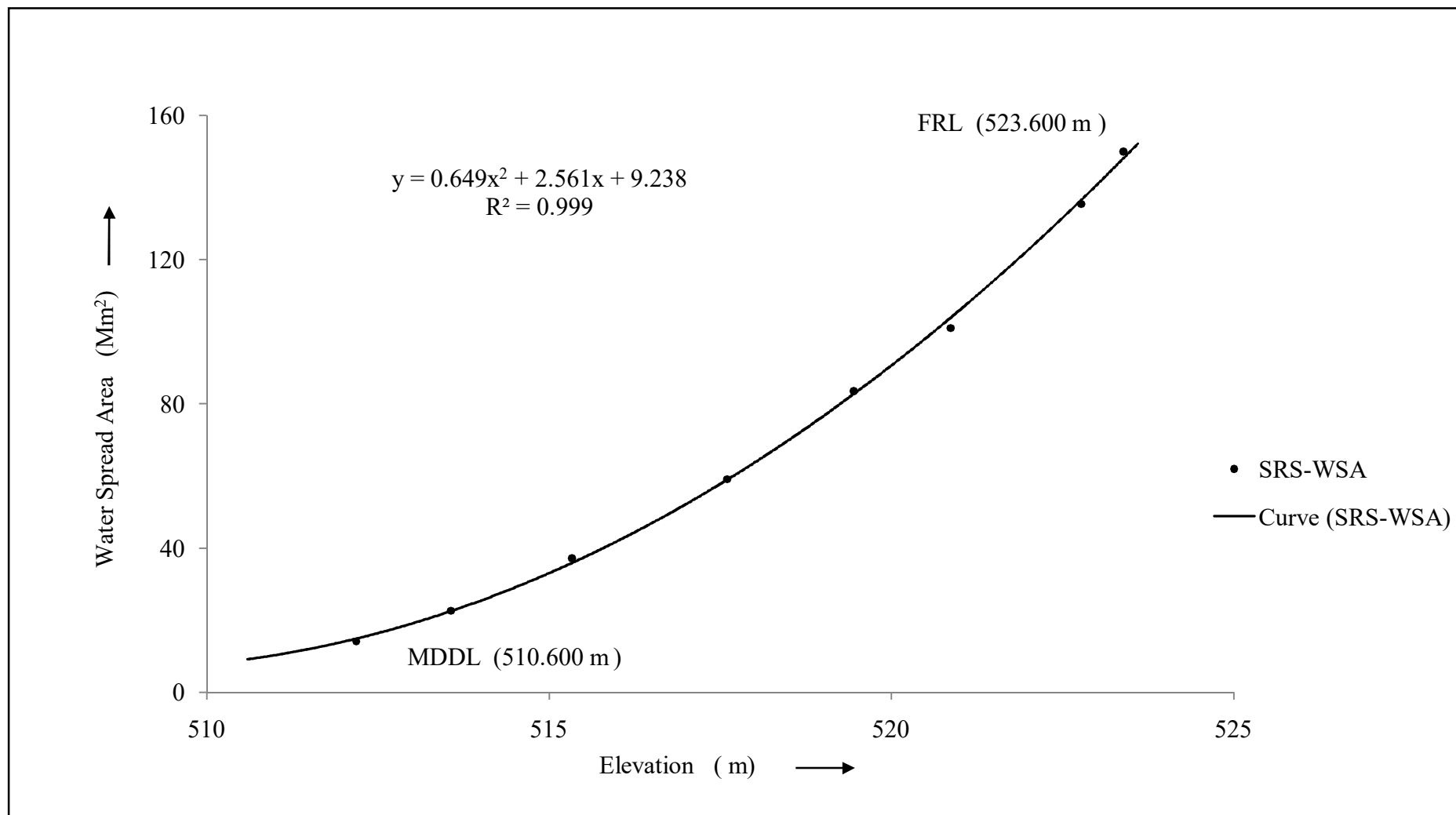
Figure 8 : SRS Elevation-Area curve for Singur reservoir, Telangana
